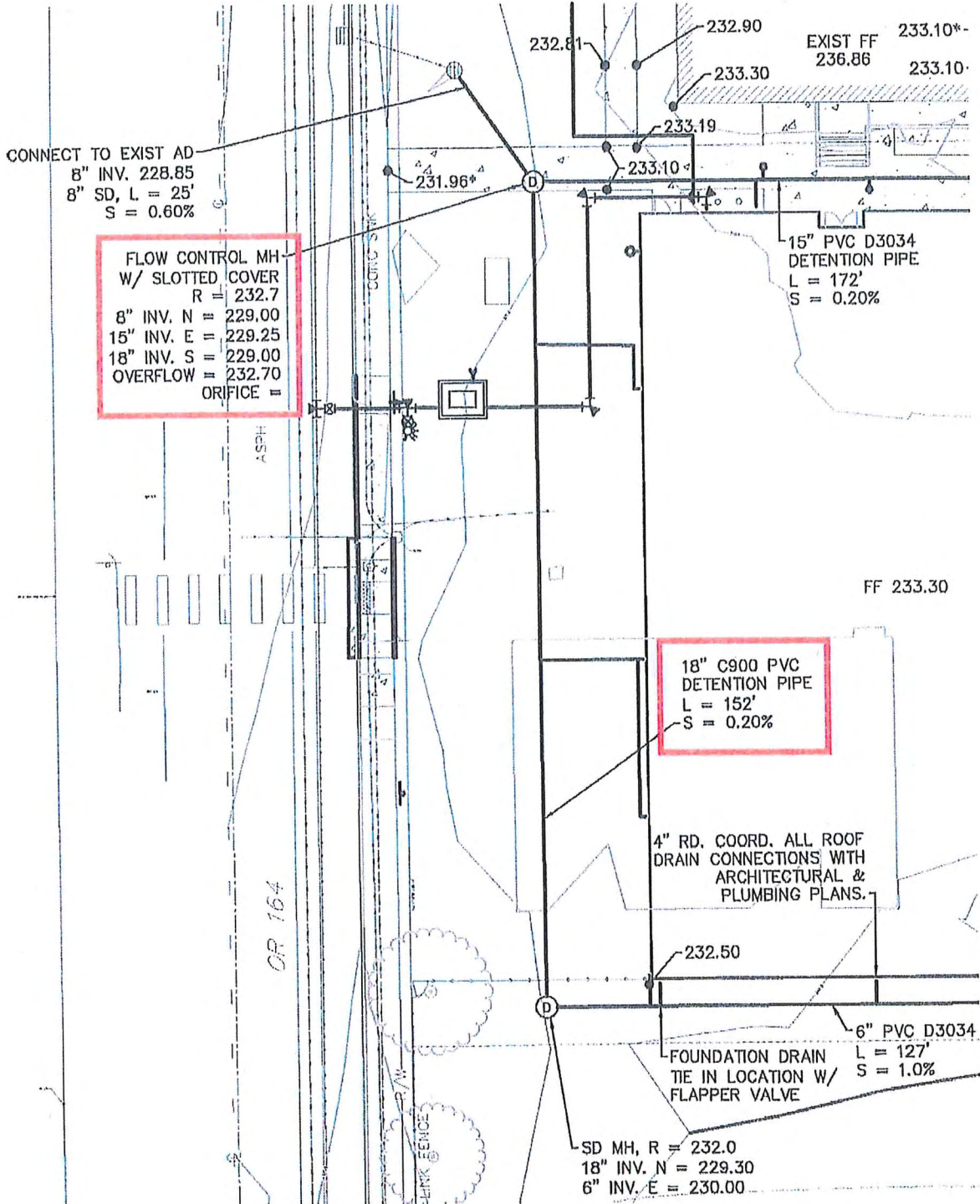
Figure 5-7 | Pipe Detention
