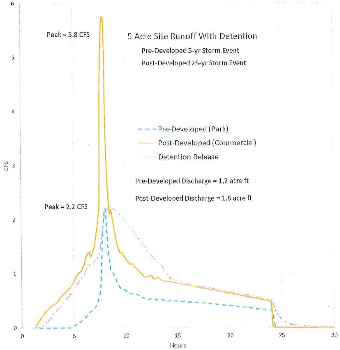
Figure 5-5 | Site Runoff With Detention
