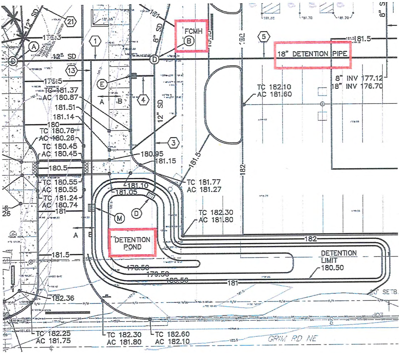
Figure 5-6 | Combined Landscape Area Detention and Pipe Detention
