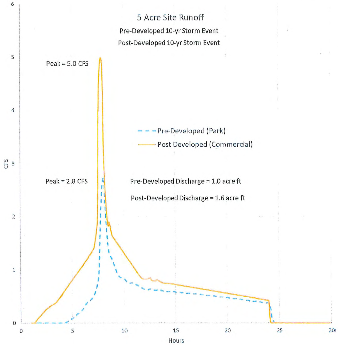
Figure 5-4 | Pre & Post Development Runoff
