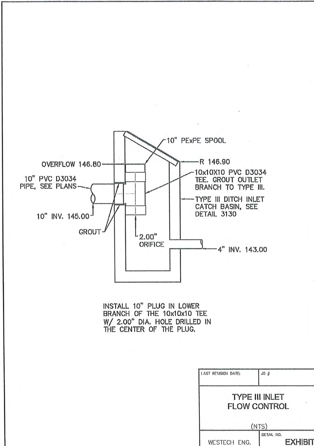
Figure 5-11 | Flow Control Type III Inlet
