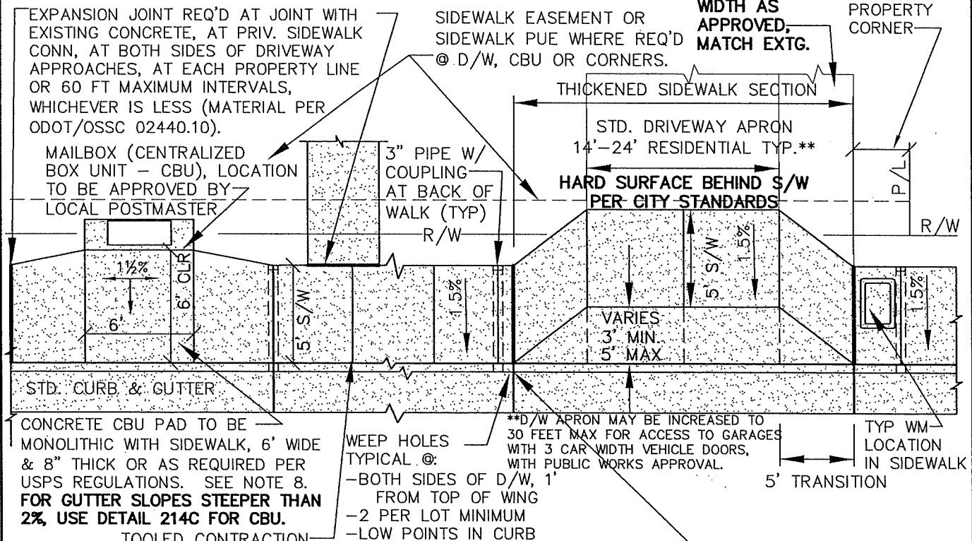
TYP. PLAN VIEW
