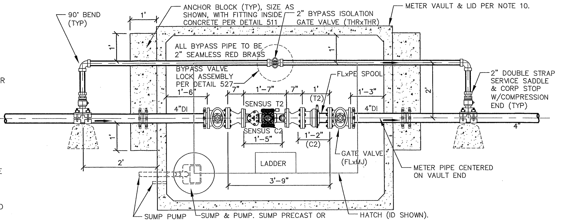
PLAN NTS
