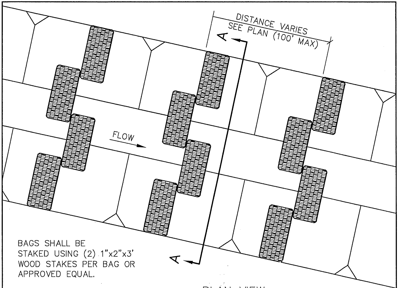
PLAN VIEW
