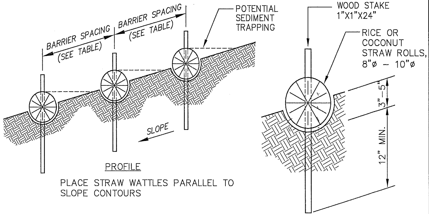
SECTION
