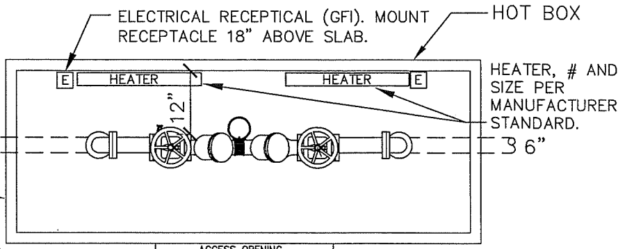
PLAN NTS
