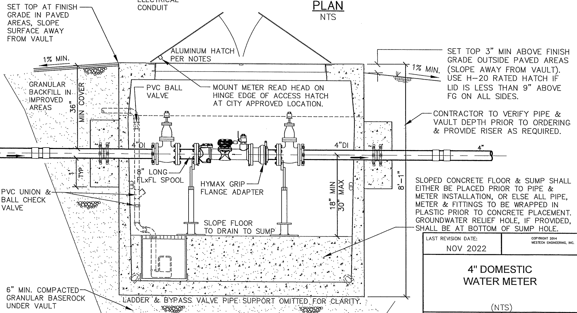
SECTION NTS
