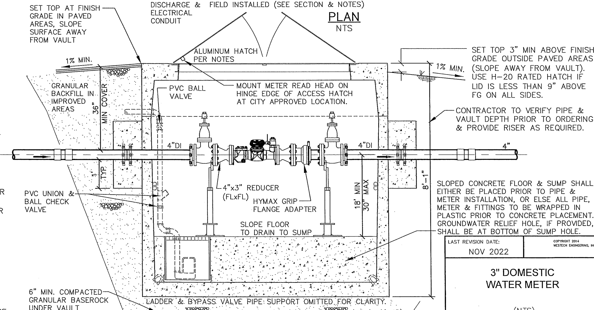
SECTION NTS
