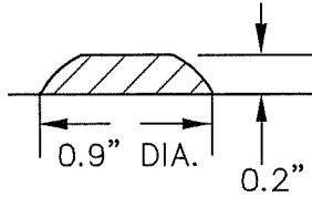
DOME PROFILE
