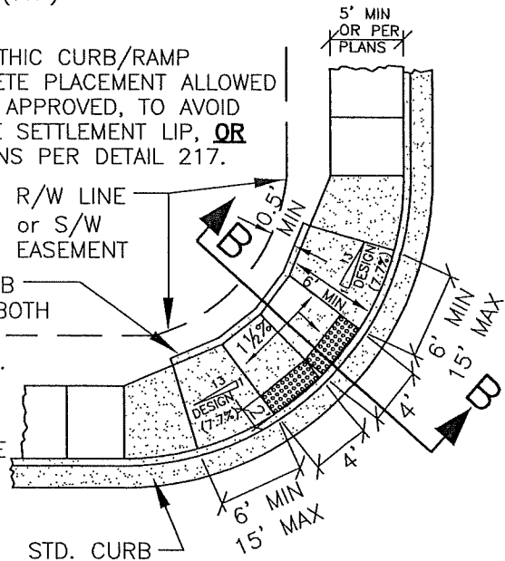
GUTTER SLOPE AROUND RADIUS 2% MAX (SEE SECTION B)
