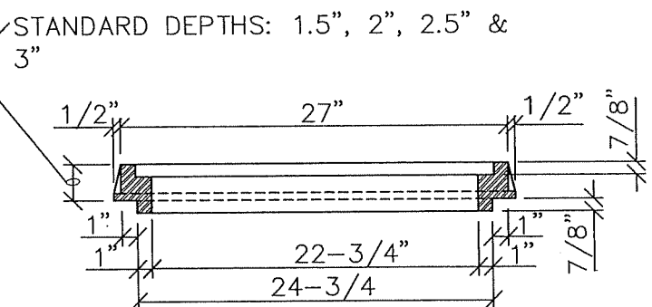
CAST IRON ADJUSTMENT RINGS
