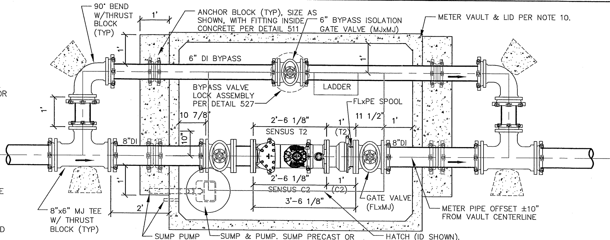
PLAN NTS
