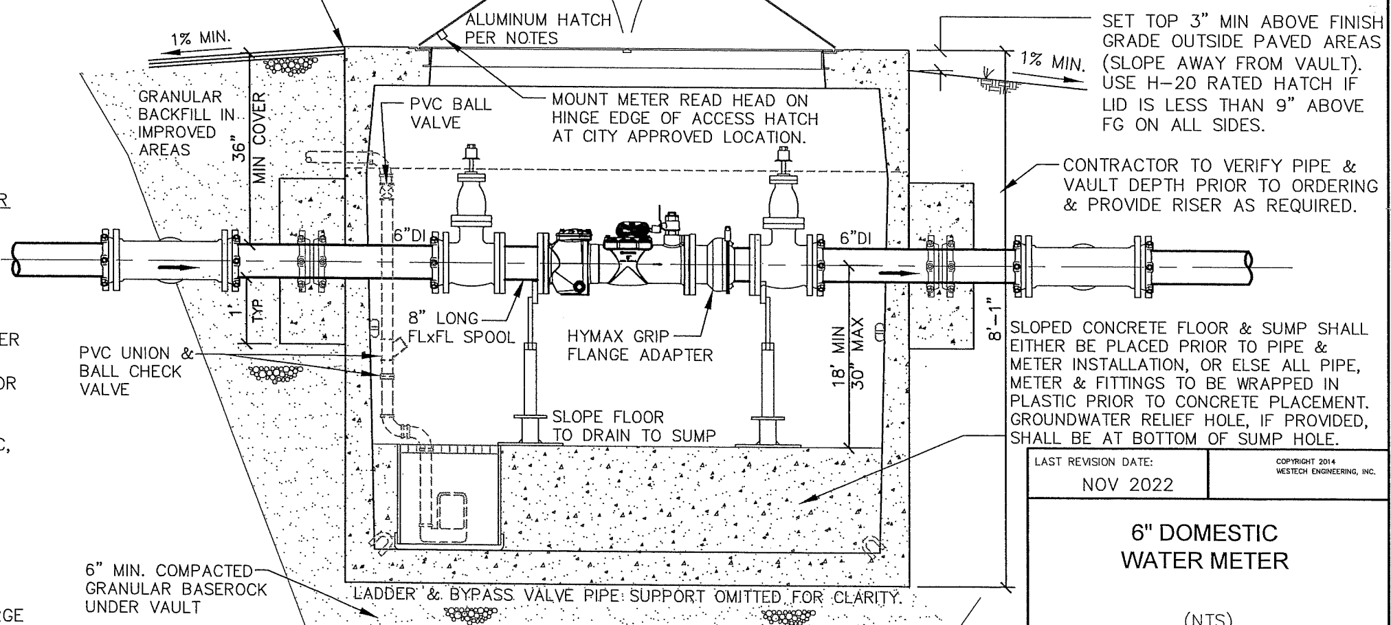
SECTION NTS
