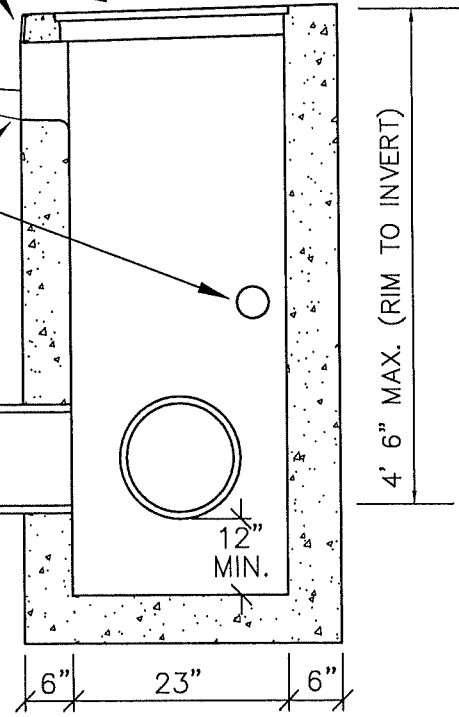
SECTION B-B
