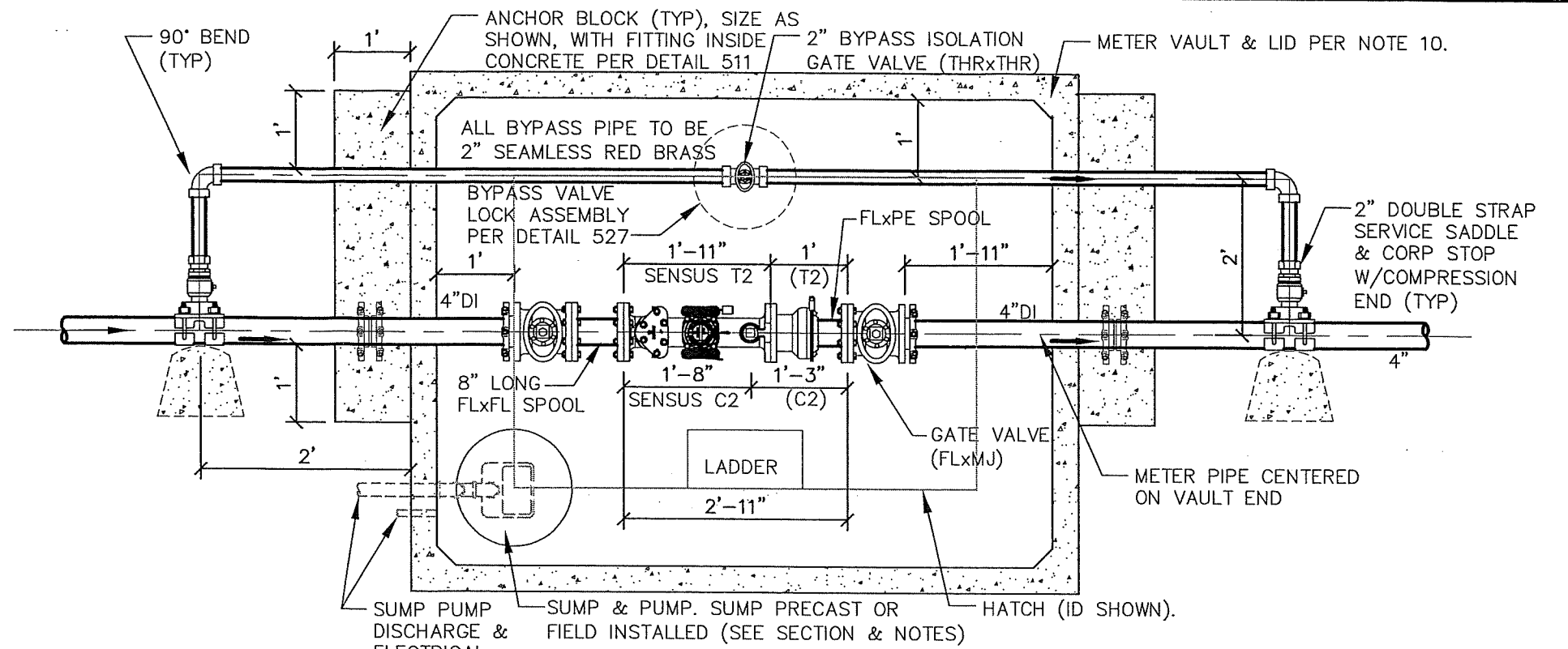
PLAN NTS
